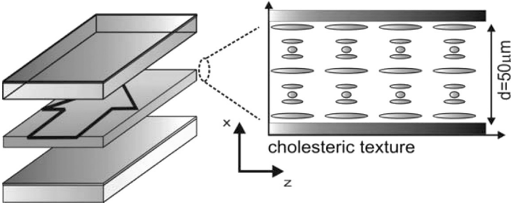
FIGURE 1 Configuration of the analyzed chiral nematic liquid crystal cell.
