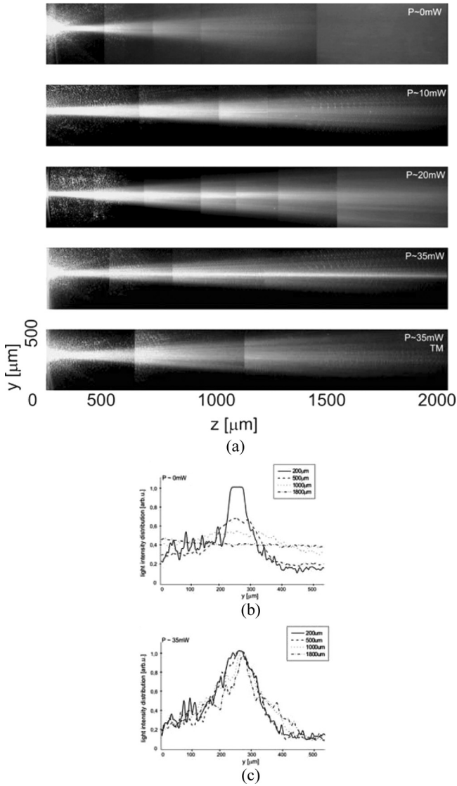
FIGURE 3 Experimental results of creation spatial solitons in ChNLCs layer; (a) light beam propagation for different inputs of light power (marked on photos) and centrally launching light beam, the last picture was taken for the TM polarization, (b)–(c) light intensity profiles for low and high power respectively, and for different values of propagation distance, corresponding to photos from (a).
