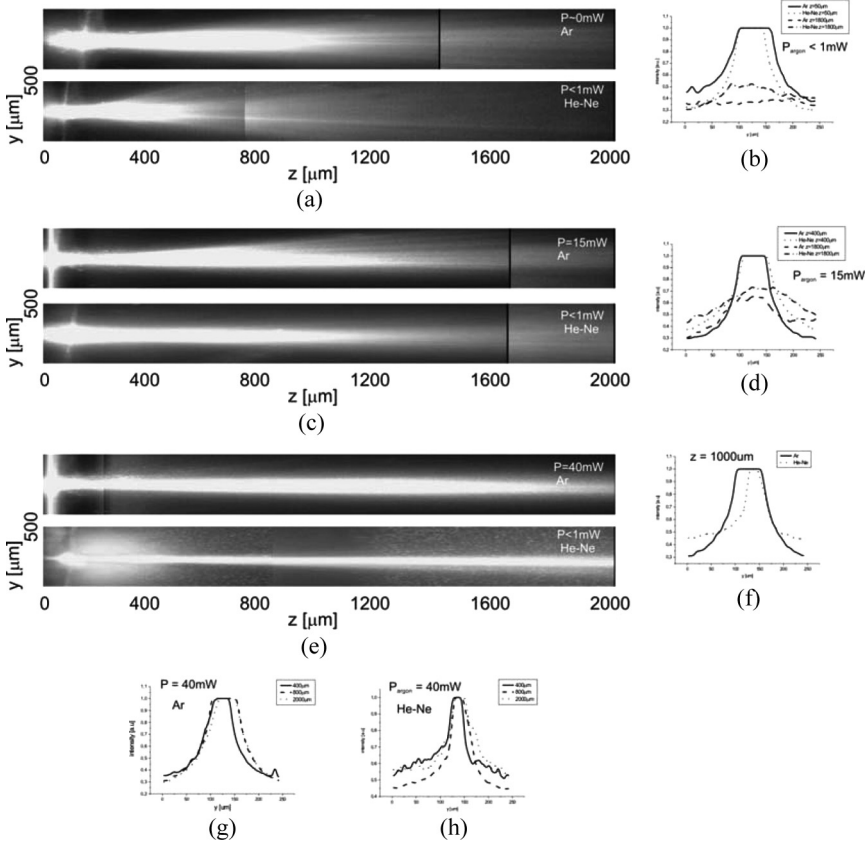
FIGURE 5 Propagation of the He - Ne low-power probe beam in the waveguide induced by the Ar beam and corresponding normalized intensity profiles at different propagation distances in the linear diffraction case (a), (b), for the Ar beam power P = 15 \text{ mW} (c), (d) and for P = 40 \text{ mW} (e)–(h).
