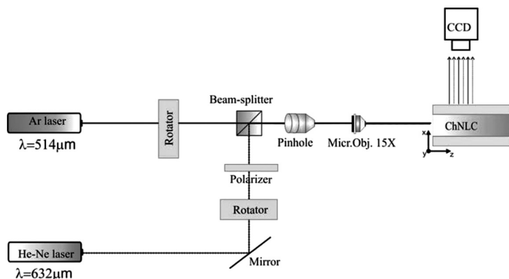
FIGURE 4 Schematic drawing of the experimental layout for two-beam measurements.
