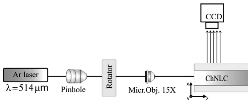
FIGURE 2 Schematic drawing of the experimental setup.
